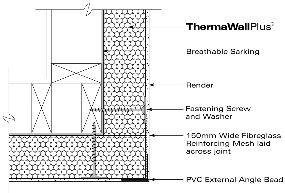
External Corner
