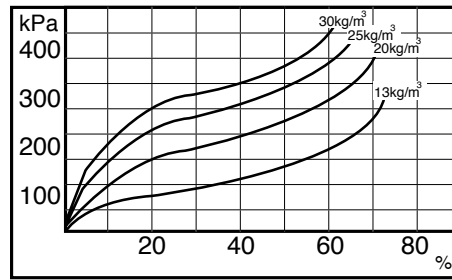
Figure 5: Stress v compressive strain
