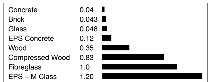
Figure 8: Typical R-values, various insulating materials 50mm thick
