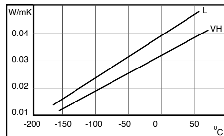
Figure 9: Indicative thermal conductivity v temperature
